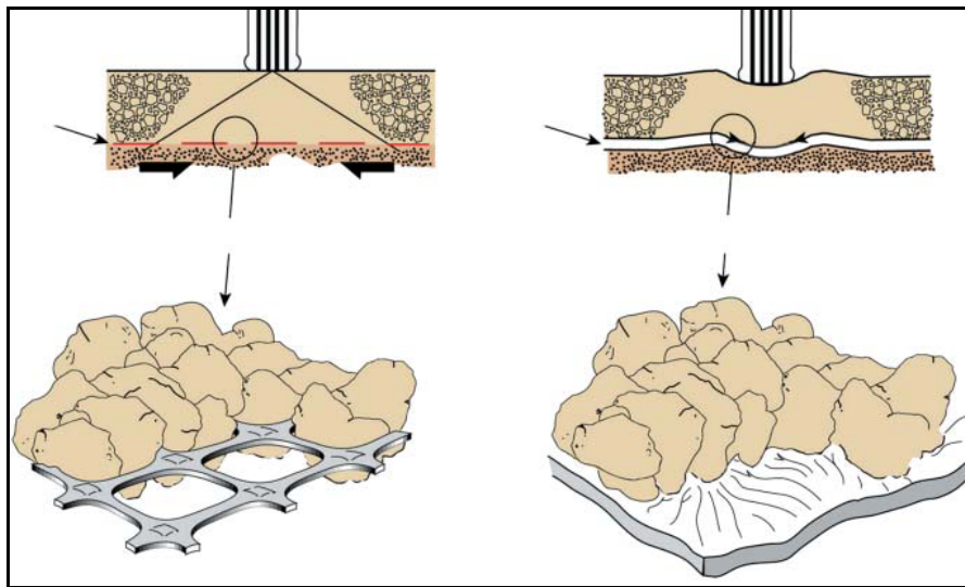
Figure 8 – Confinement Effect – Biaxial Geogrid vs Tensioned Membranes
