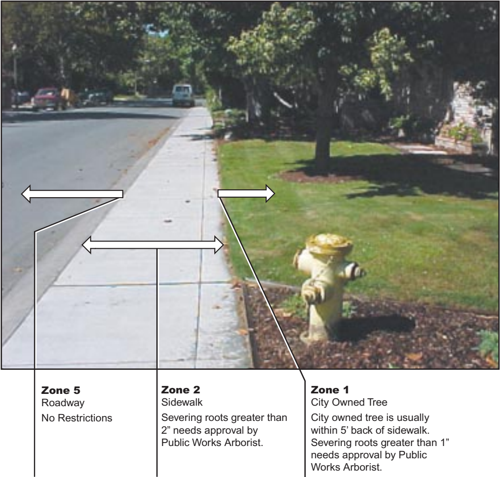
IMAGE 2.20-3 Restriction Zones for Excavation, Trenching or Boring within a Tree Dripline behind Sidewalk and Rolled Curb
