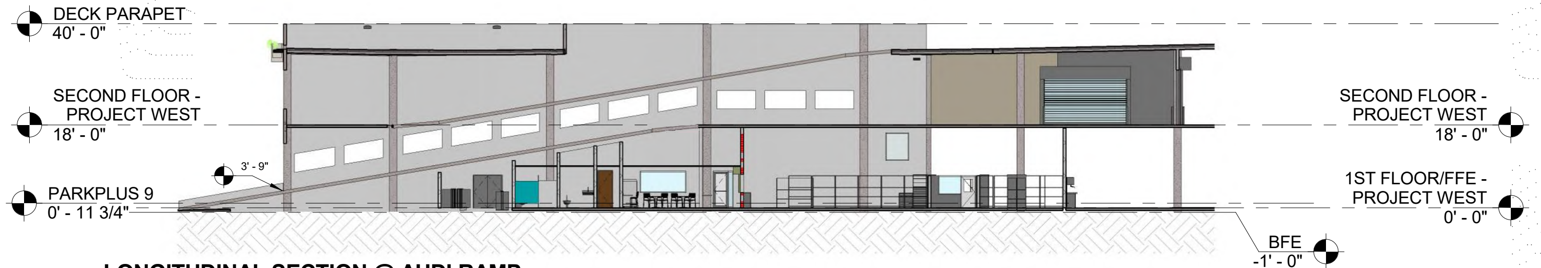
LONGITUDINAL SECTION @ AUDI RAMP
