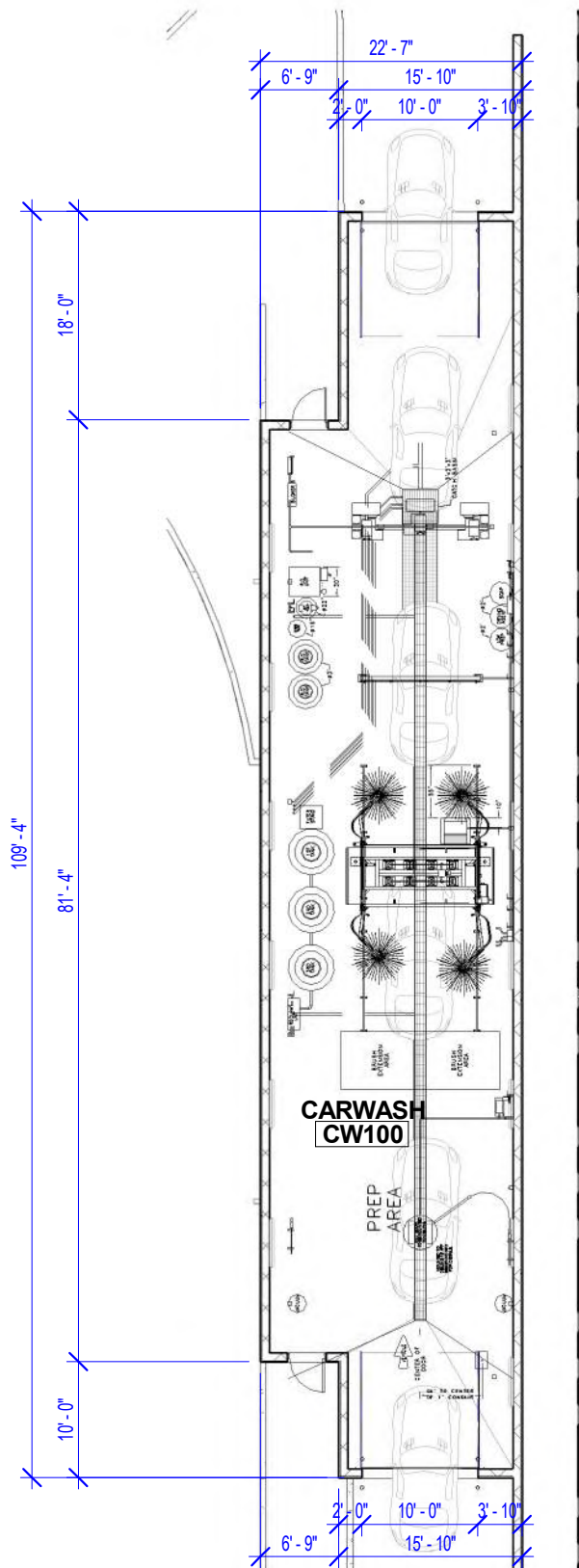
FLOOR PLAN - CAR WASH
