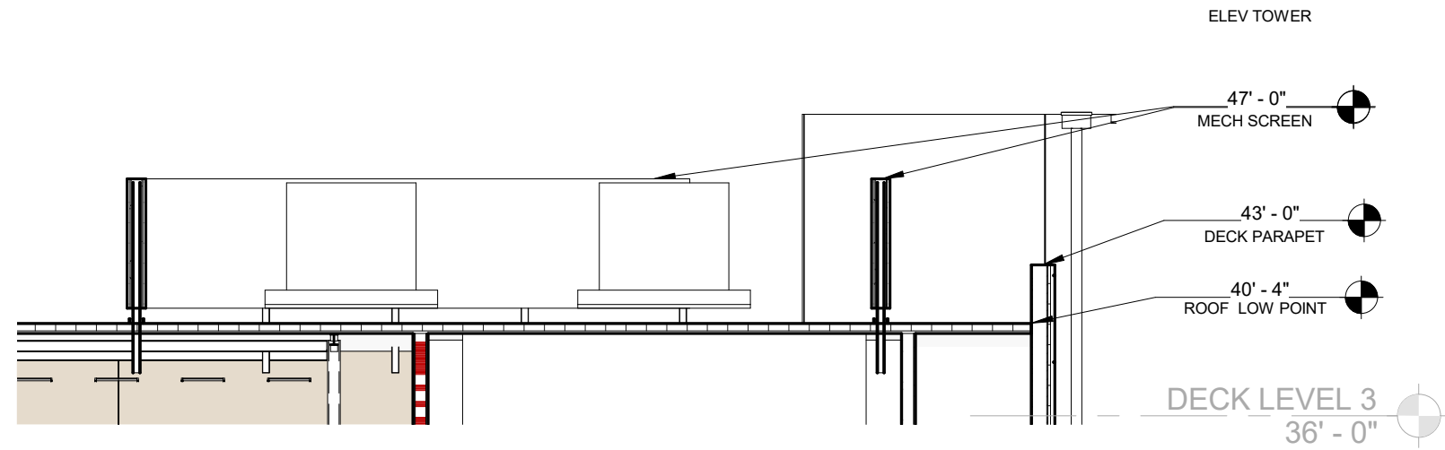
MECH SCREEN SECTION @ MB
