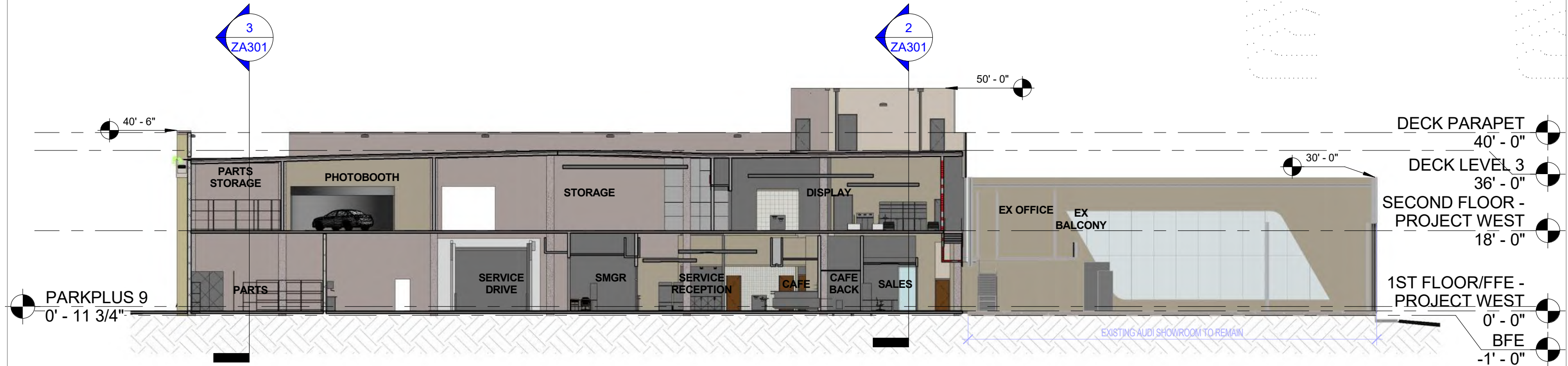
LONGITUDINAL SECTION @ AUDI SHOWROOM
