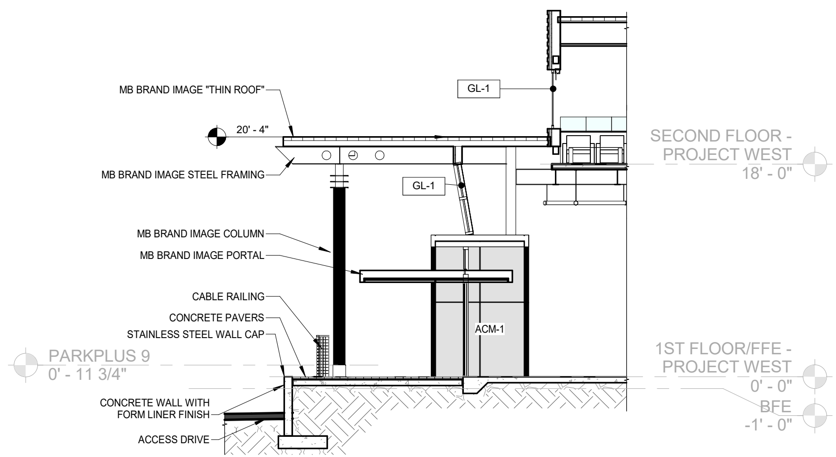
1 MB MAIN ENTRY ZA311 1/8" = 1'-0"
