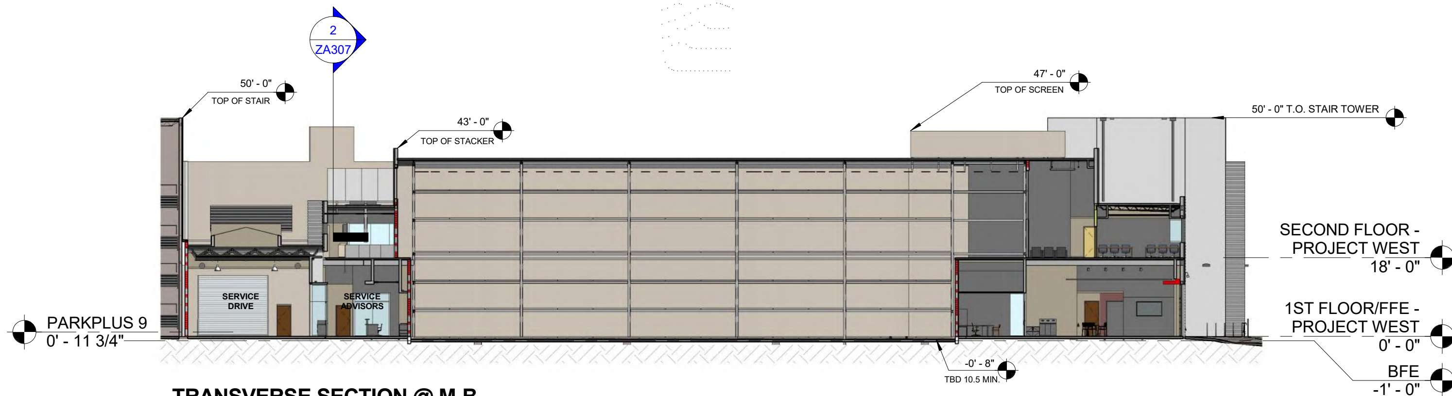
TRANSVERSE SECTION @ M-B 3/64" = 1'-0"
