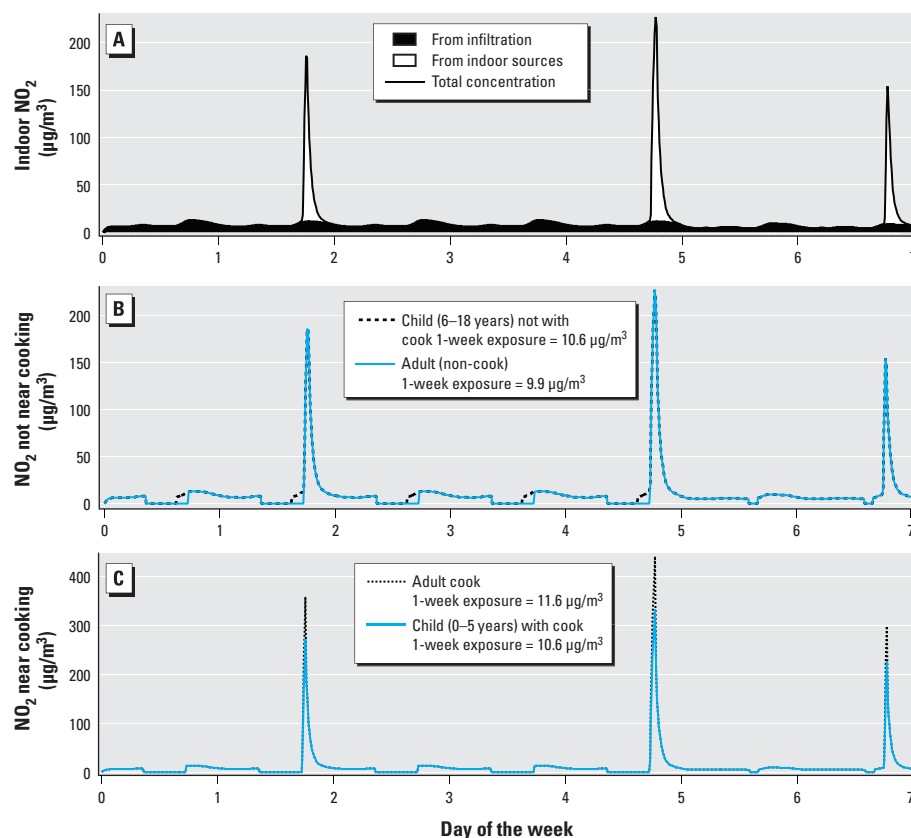
Figure 1. Example results: simulated time-resolved \text{NO}_2 concentrations in a 36-year-old, 1,125-ft 2 home with four occupants (one 0–5, one 6–18, and two 35–54 years of age) for 1 week in winter. (A) Indoor concentration of \text{NO}_2 originating from indoor and outdoor sources. (B) Simulated exposure concentration experienced by the two occupants assumed to not be near the cooking activity ( F_{\text{prox}} = 1 ). (C) Simulated exposure concentration for the cook ( F_{\text{prox}} = 2 ) and a small child assumed to be near the cooking ( F_{\text{prox}} = 1.5 ).
