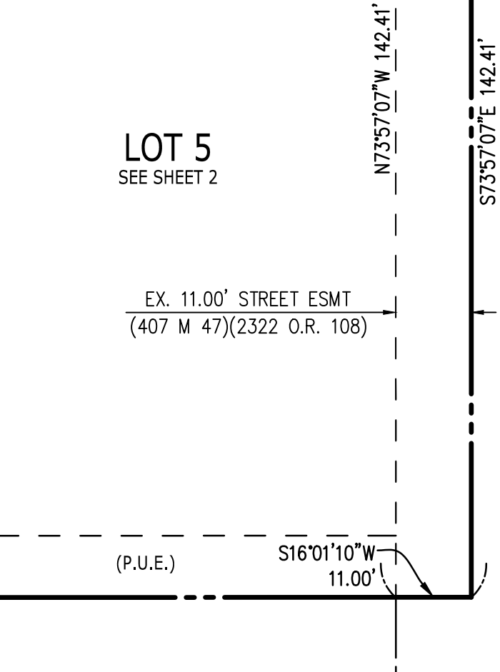
DETAIL C SCALE: 1"=20'
