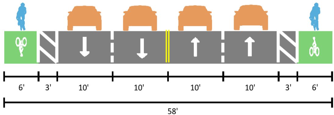
Option 1 Buffered Bike Lanes | Opción 1 Ciclo Carriles
