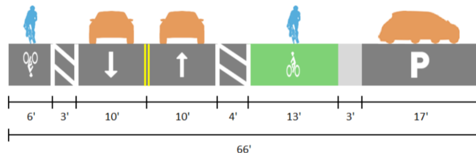
Option 1 Buffered Bike Lanes | Opción 1 Ciclo Carriles
