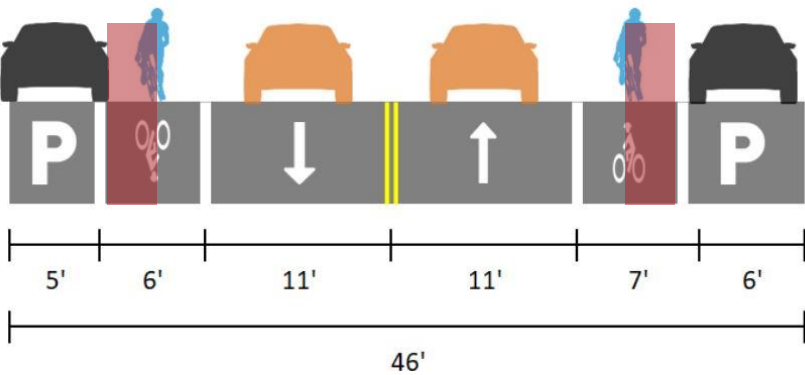
Option 1 Buffered Bike Lanes | Opción 1 Ciclo Carriles
