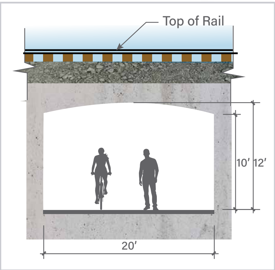
3 Section Through Tunnel
