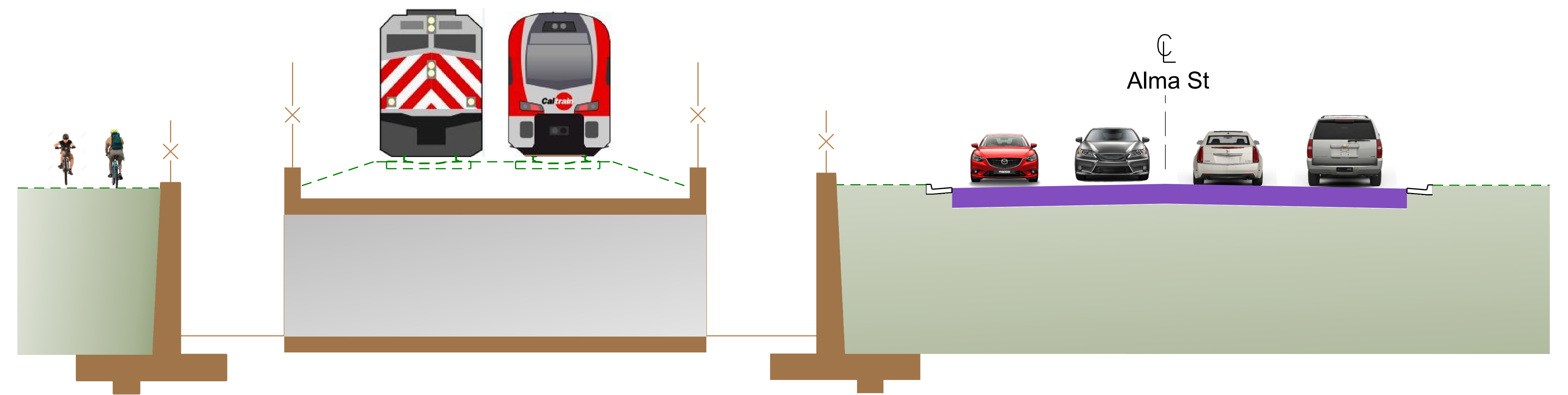
Section B-B
