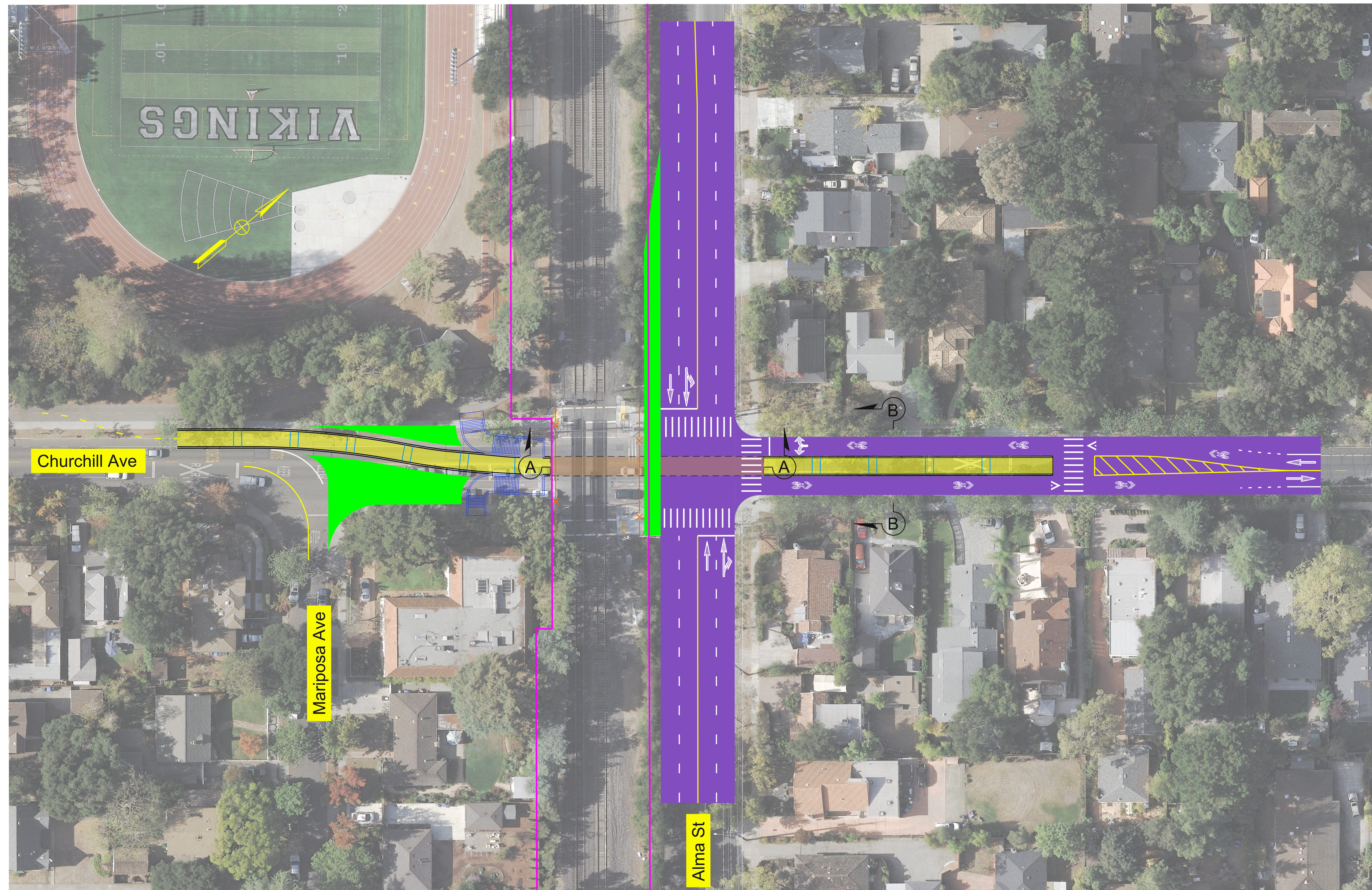
Churchill Avenue (Plan)
