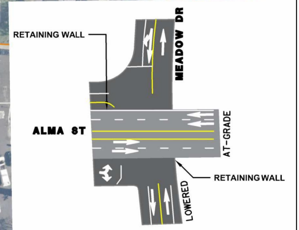
INTERSECTION TURNING MOVEMENT DIAGRAM
