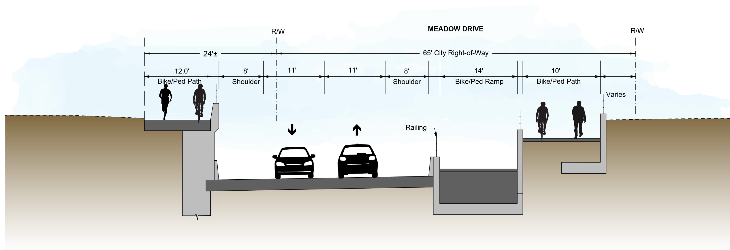
MEADOW DRIVE UNDERPASS MEADOW DRIVE CROSS-SECTION
