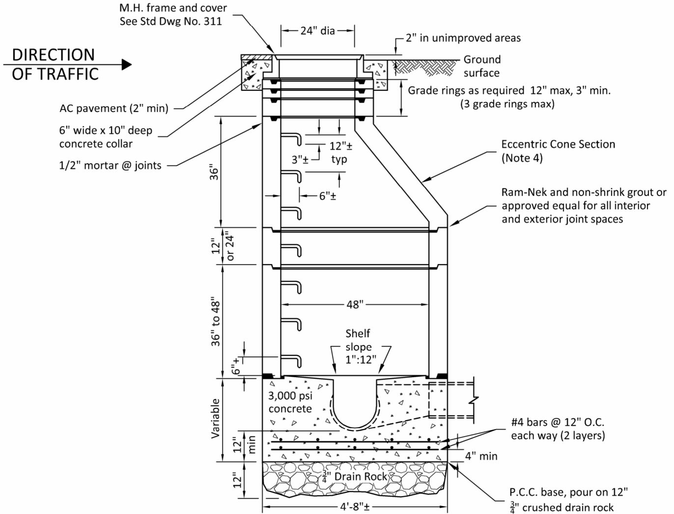
SECTION
